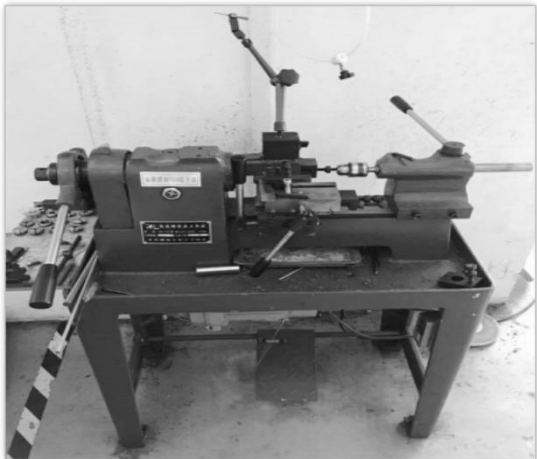
Instrument lathe [1]
